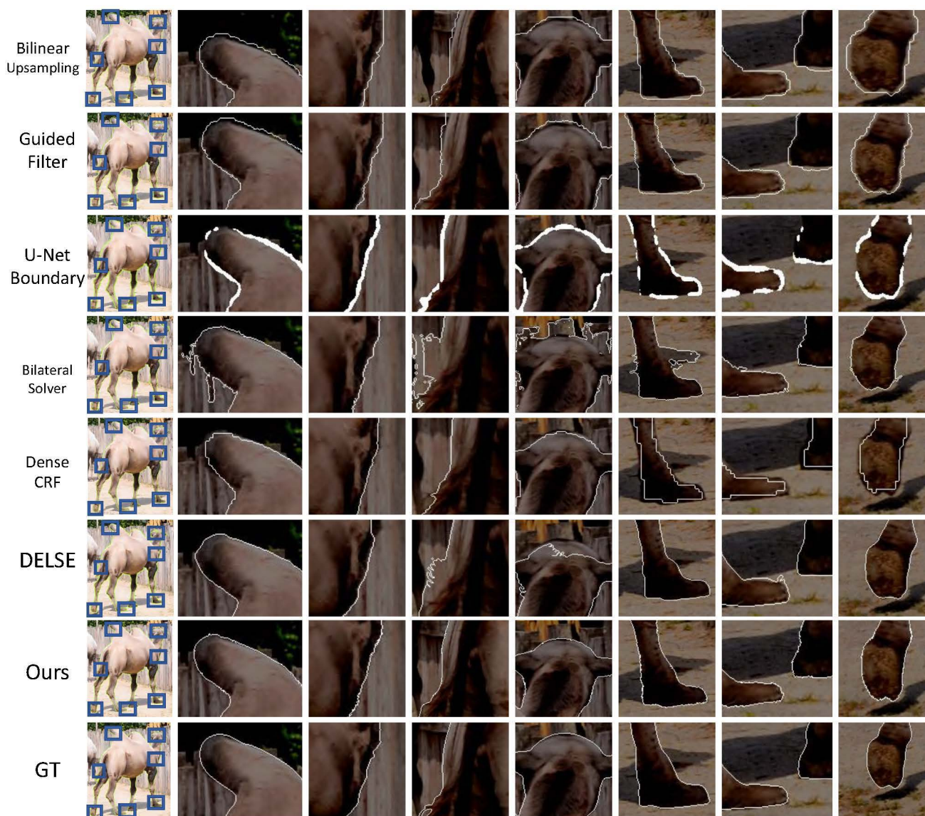
Figure 8. Multi-region visualization on DAVIS 2016. The first column shows the whole image and the rest columns are the enlarged box regions. Boundaries are highlighted in white. Notice that our approach has closer prediction than methods like bilinear upsampling and guided filter, has less spurious boundaries than DELSE and bilateral solver, and thinner boundaries than U-Net Boundary.
