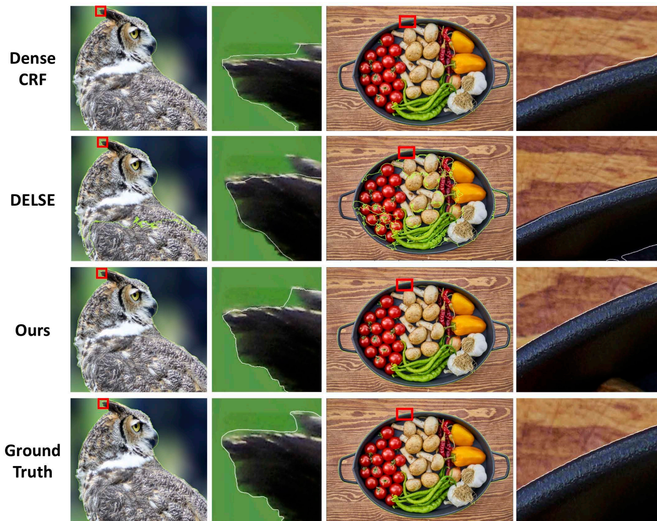
Figure 12. Additional visualization on PixHR 16 \times . We first show the whole boundary visualization and then show the enlarged box region. The boundaries in the enlarged regions are displayed in white. Notice that our approach makes smoother prediction than dense CRF and less false positive than DELSE.
