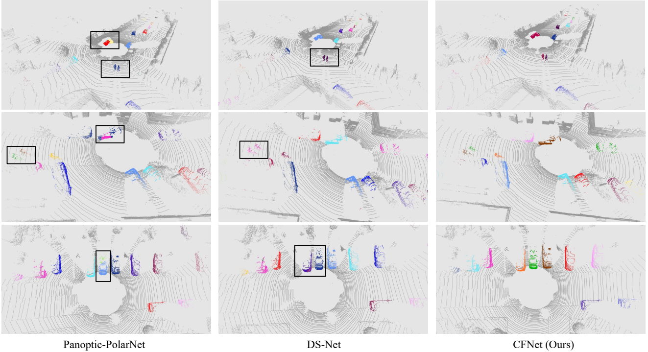
Figure 9. Comparison visualization results of the instance segmentation from the Panoptic-PolarNet [39], DS-Net [15], and our CFNet on the SemanticKITTI test set. The black box marks the region of interest.
