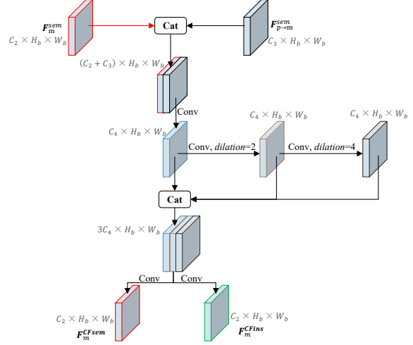
Figure 6. The feature enhancement module in the proposed CFFE. “Conv” represents a 2D convolution with 3 \times 3 kernels, a batch normalization, and a ReLU layer. dilation denotes the dilation coefficient of the 2D convolution and is set as 1 unless specified.
