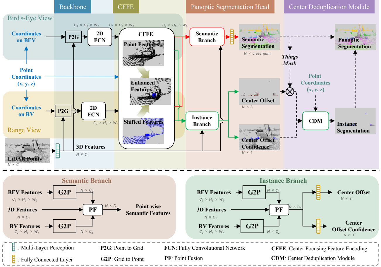
Figure 7. The overview of our CFNet with the backbone of the CPGNet [23].
