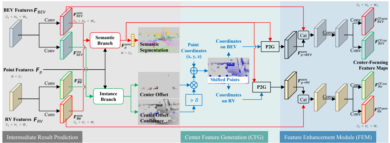
Figure 8. The proposed center focusing feature encoding (CFFE) that is integrated with the CPGNet [23] backbone. The “Conv” represents a 2D convolution with 3 \times 3 kernels, a batch normalization, and a ReLU layer. The details of the semantic branch and instance branch are shown in Fig. 7. The blue arrows are coordinate-related operations.
