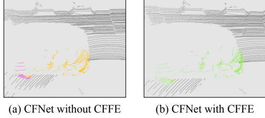
Figure 2. Instance segmentation of a car. Without our CFFE, the car is split into parts (a), while the CFFE significantly alleviates this problem (b). Different colors represent different instances.
