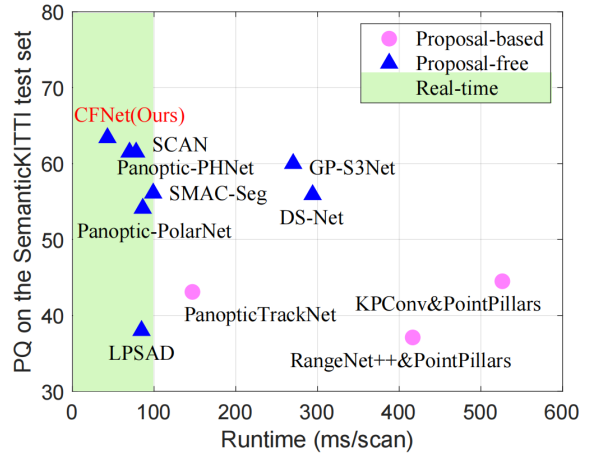
Figure 1. PQ vs. runtime on the SemanticKITTI test set. Runtime measurements are taken on a single NVIDIA RTX 3090 GPU. The panoptic quality (PQ) is introduced in section 4.1.
