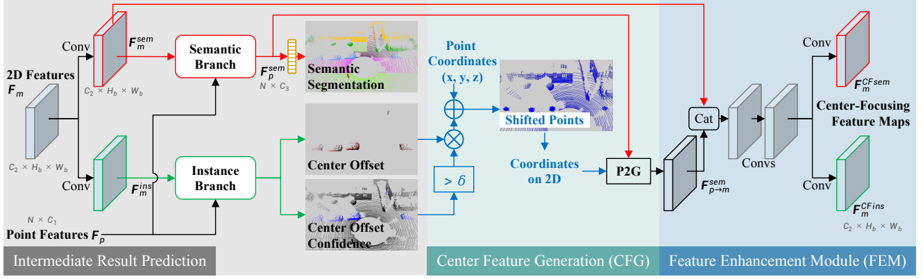
Figure 4. The proposed center focusing feature encoding (CFFE). The “Conv” represents a 2D convolution with 3 \times 3 kernels, a batch normalization, and a ReLU layer. The details of the semantic branch and instance branch are shown in Fig. 3. The blue arrows are coordinate-related operations.
