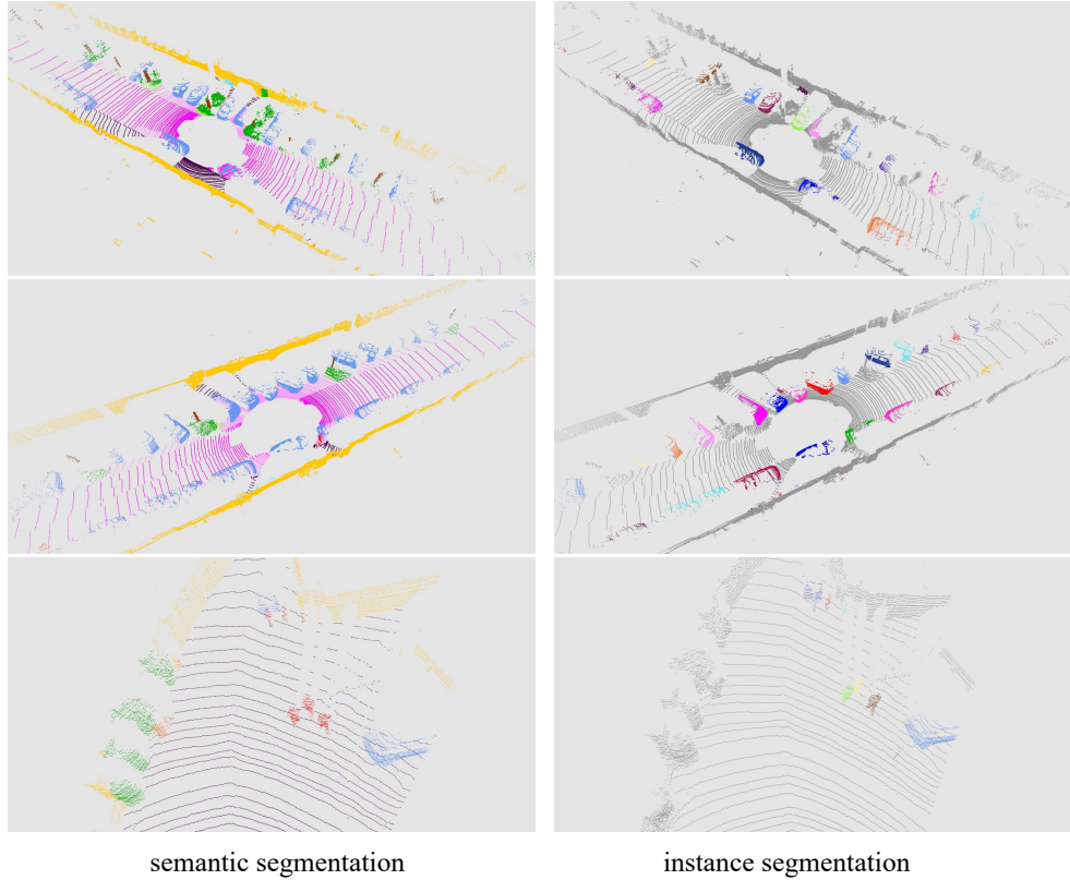
Figure 10. Visualization results of our CFNet on the SemanticKITTI test set. For semantic and instance segmentation, different colors represent different classes and instances, respectively.
