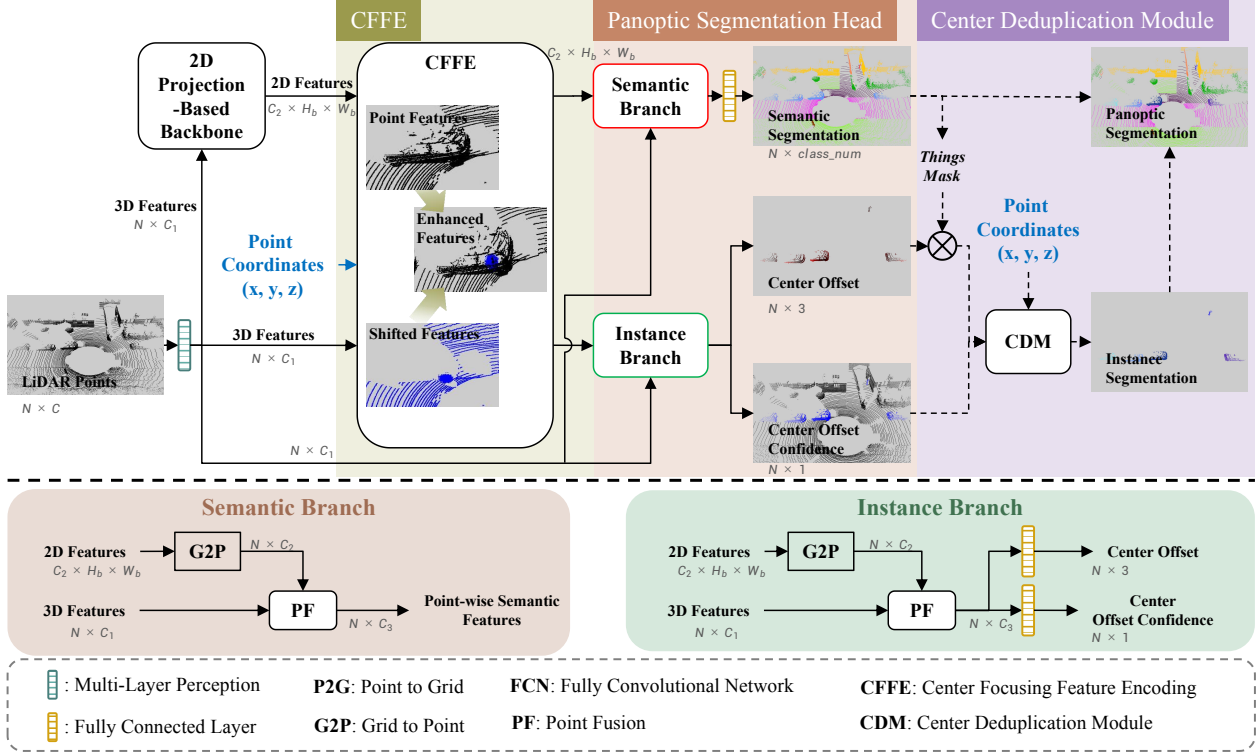
Figure 3. The overview of our CFNet. It consists of four steps: 1) the 2D projection-based backbone extracts features on the 2D space; 2) the proposed center focusing feature encoding (CFPE) mimics and enhances the non-existent instance center features; 3) the panoptic segmentation head predicts the output results; 4) the proposed center deduplication module (CDM) achieves instance segmentation that is fused to generate the final panoptic segmentation results. The dashed lines indicate that the operations are only used during inference.
