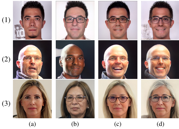
Figure 3. Qualitative comparison among different compositional manipulation methods on real image inputs. Target attributes from the top row to the bottom row are (1) glasses, smile, 55 y/o, (2) no glasses, smile, 28 y/o, (3) glasses, white hair, right face. Each column from left to right are (a) original images, (b) LACE-ODE [27], (c) linear latent classifier guidance in \mathcal{W}_s , (d) linear latent classifier guidance in \mathcal{W}_s+ .
