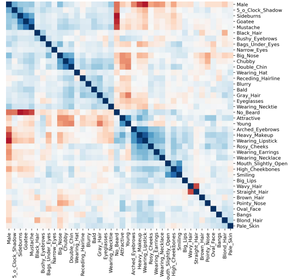
Figure 4. Visualization of Latent semantic correlations of Diffusion Autoencoder. Bluer regions indicate positive correlations and redder areas suggest negative correlations.
