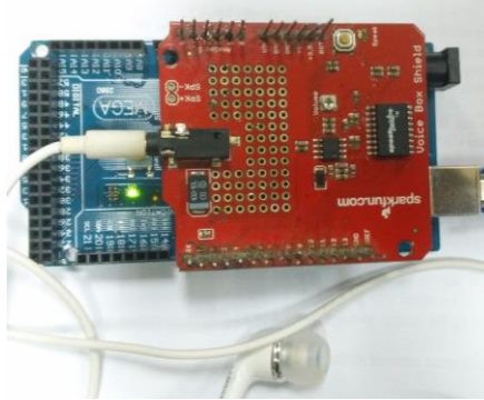
Fig 8 Voice Box Shield
