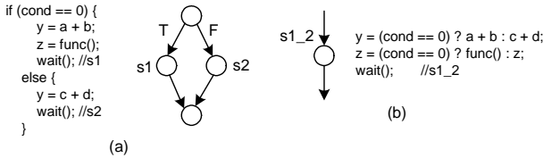
Figure 4. Predicate conversion.
