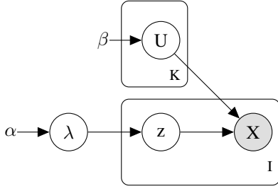
Fig. 2. The latent class model in plate notation. Each node represents a random variable and X is shaded gray because it is the only variable which is observed. The arrows represent the dependency structure and the plates represent repeated values. K means that we have one U_k for each cluster 1 to K . Analogous we have one cluster assignment and the corresponding set of observation for each individual 1 to I . \lambda is the cluster size proportion and drawn from a Dirichlet( \alpha ).
