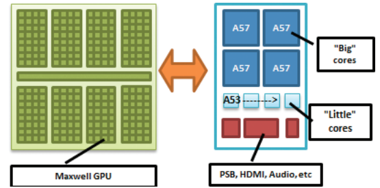
Fig. 1. Scheme of the NVIDIA Tegra X1 platform
