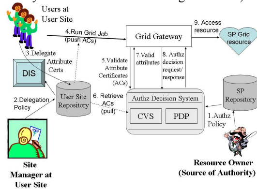
Figure 2: The Delegation/Authorisation Model
