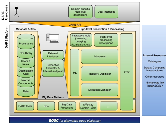
Fig. 1. Overview of the DARE platform.
