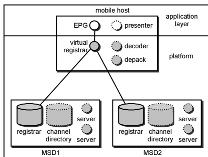
Figure 2. Registration service.
