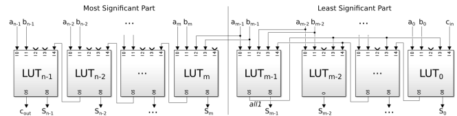
Fig. 1: Approximate adder implemented with LUTs as available on FPGAs. It makes use of the not connected inputs of the 5 \times 2 LUTs provided in Xilinx 7-series devices in order to reduce the error generated by disconnecting the carry chain. This can be done on occasions where a carry would be produced at m - 1 but is not forwarded to LUT_m . By simply connecting the bits at LUT_{m-2} to LUT_{m-1} , an all1 signal can be generated and forwarded to the lower bits, setting their outputs to 1. Furthermore, bits m - 1 are connected to LUT_m in order to allow correct carry propagation if bits m - 1 are both 1 reducing the error drastically.
