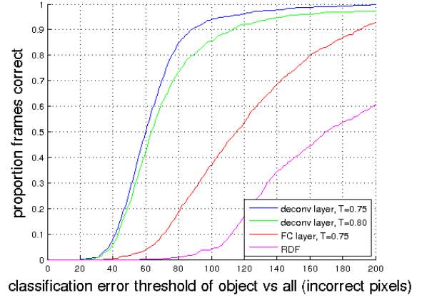
Fig. 4: Evaluation of stage one, the hand-object segmentor.
