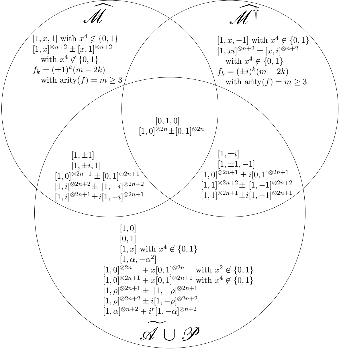
Figure 36: A Venn diagram of the Pl-#CSP 2 tractable sets \widehat{\mathcal{M}} and \widehat{\mathcal{M}}^\dagger along with the set \widetilde{\mathcal{A}} \cup \mathcal{P} of all tractable #CSP 2 signatures. Note that \rho^4 = 1 , \alpha^4 = -1 , and n \geq 1 . Excluded are tensor products of unary signatures.
