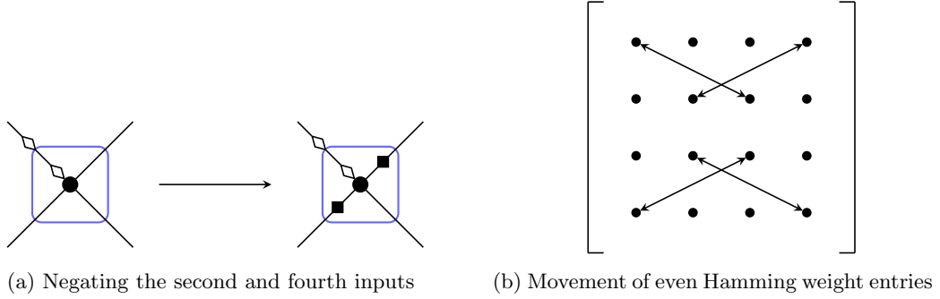
Figure 9: The movement of the even Hamming weight entries in the signature matrix of a quaternary signature under the negation of the second and fourth inputs (i.e. the square vertices are assigned [0, 1, 0] ).
