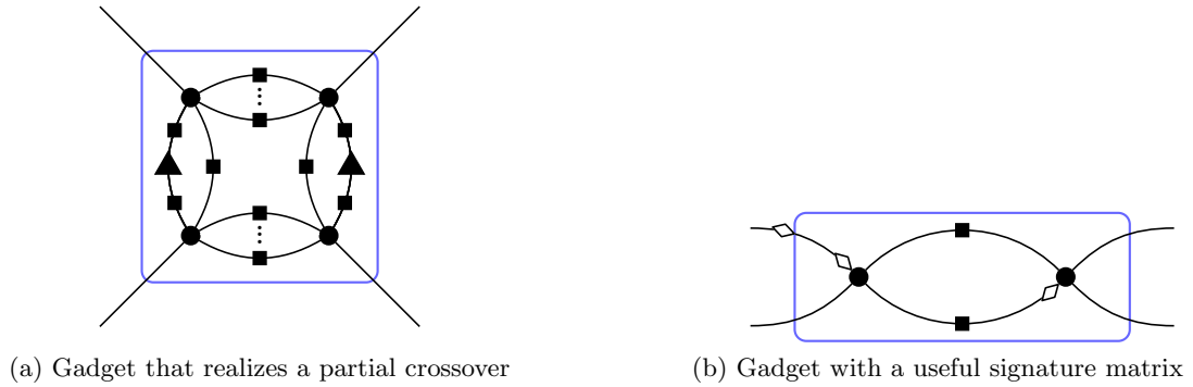
Figure 10: Two quaternary gadgets used in the proof of Lemma 6.7 and 6.8.
