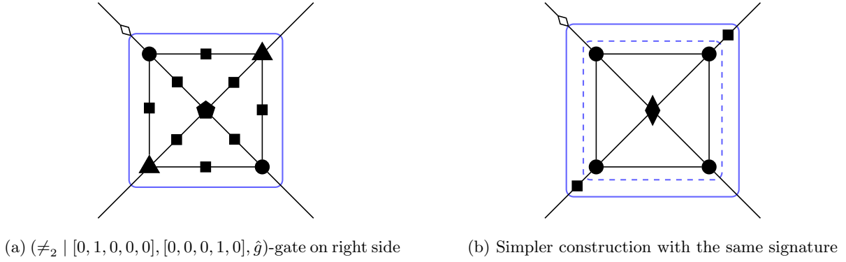
Figure 8: Two gadgets with the same signature used in Lemma 6.7.
