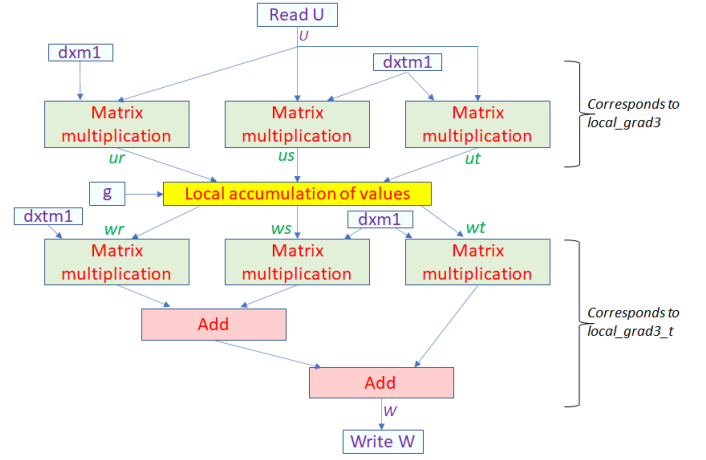
Fig. 1. Illustration of the dataflow architecture of our HLS kernel
