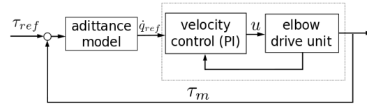
Figure 6. Control scheme
