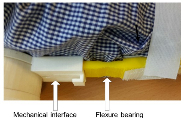
Figure 2. Forearm link with integrated flexure bearing to ensure a compliant behavior
