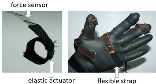
Figure 5. Force sensor protected by textile for the index finger (left), full glove (Nitras Nylontex 3520, right)
