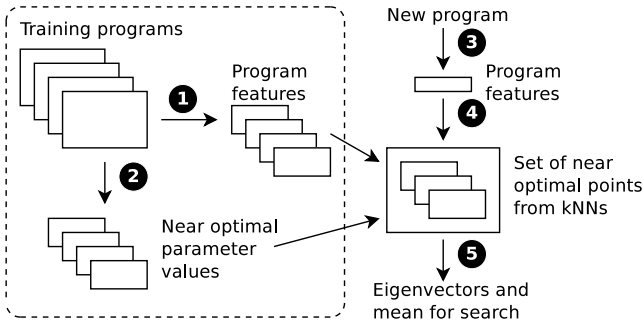
Figure 2: Schematic of how machine learning guides the search. The dotted box indicates the offline training phase. ① Extract program features from training programs. ② Find a set of near optimal parameter values for each training program, by measuring a random subset of the space. ③ Extract program features from the new program. ④ Compute the k -nearest neighbors, using the program features, to create a set of near optimal parameter values for all nearest neighbors. ⑤ Apply PCA to the set of near optimal parameter values. The resulting mean and eigenvectors are used to perform the search.
