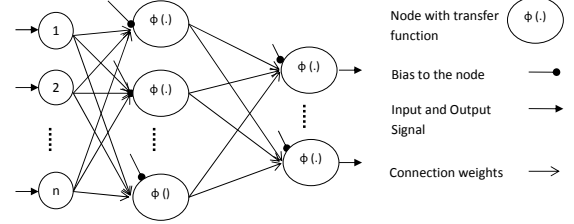
Fig. 1. Phenotype representation of NN
