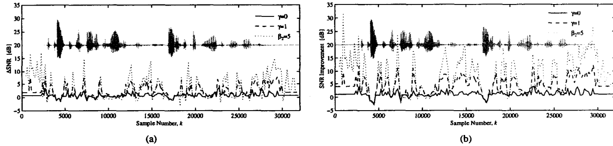
Figure 6 (a) Difference between segmental SNRs of estimates obtained by using the QSVD and SVD algorithms, i.e., \text{SNR}_{\text{QSVD}}/\text{SNR}_{\text{SVD}} . The colored noise is an AR(1,-0.7) process (global SNR=5dB). (b) Improvement in segmental SNRs for the QSVD based estimators.
