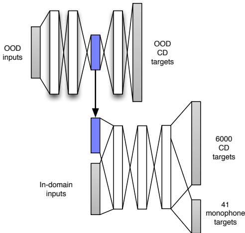
Fig. 2. Multitask network structure with MLAN features
