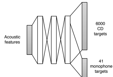
Fig. 1. Multitask network structure
