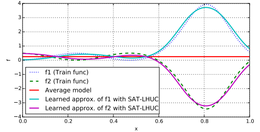
Fig. 3. Example illustration showing how SAT-LHUC can improve a learned representation. Assume we want to approximate both f_1 and f_2 with the similarly constrained (4 hidden units) model from Fig. 2. Again, it is possible with two sets of SAT-LHUC parameters for f_1 and f_2 .
