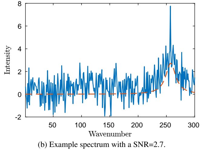
Fig. 1. Data generated by simulation. The blue line is an example spectrum with added noise and the dotted red is the true underlying spectrum.
