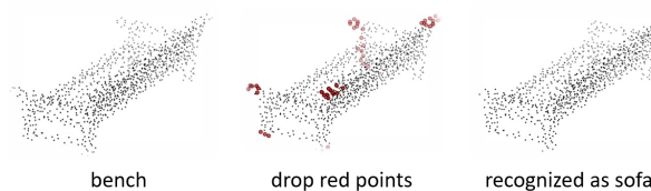
Figure 1. Drop the 5% most critical points identified by our saliency map from a bench point cloud can easily change the prediction outcome (even can trick human vision!).
