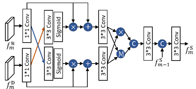
Fig. 3 Cross-enhanced integration module (CIM). C, +, \times , and M denote feature concatenation, element-wise addition, multiplication, and maximization, respectively.
