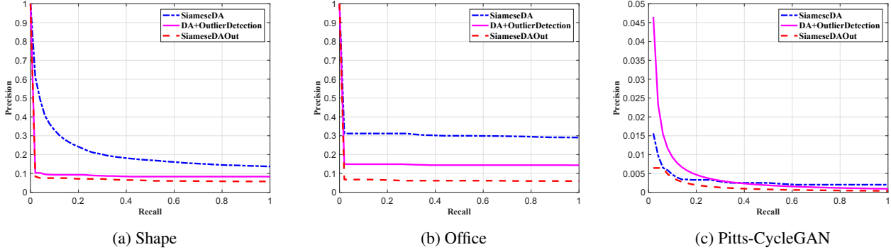
Figure 4: Precision-Recall results of our method DA+OutlierDetection , SiameseDA and SiameseDAOOut for the experiment of cross domain image matching with outlier detection on the three datasets. Our method gains over the lower bound method.
