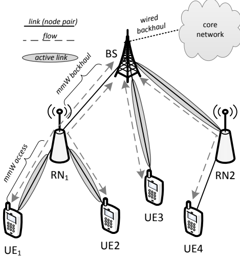
Figure 1: Directional multi-hop cellular network with millimeter wave backhaul and access links
