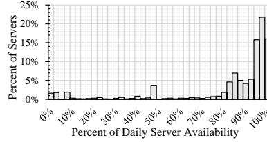
Figure 14: The distribution of servers by percent they are online over a typical day.
