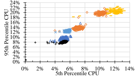
Figure 3: Scatter plot of the high and low CPU usage for each server in pool I. Shapes are datacenters.
