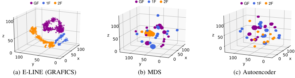
Fig. 6. The E-LINE’s embeddings of the RF signal samples from each floor naturally form a cluster in the embedding space, while MDS and autoencoder lead to poor embedding performance.
