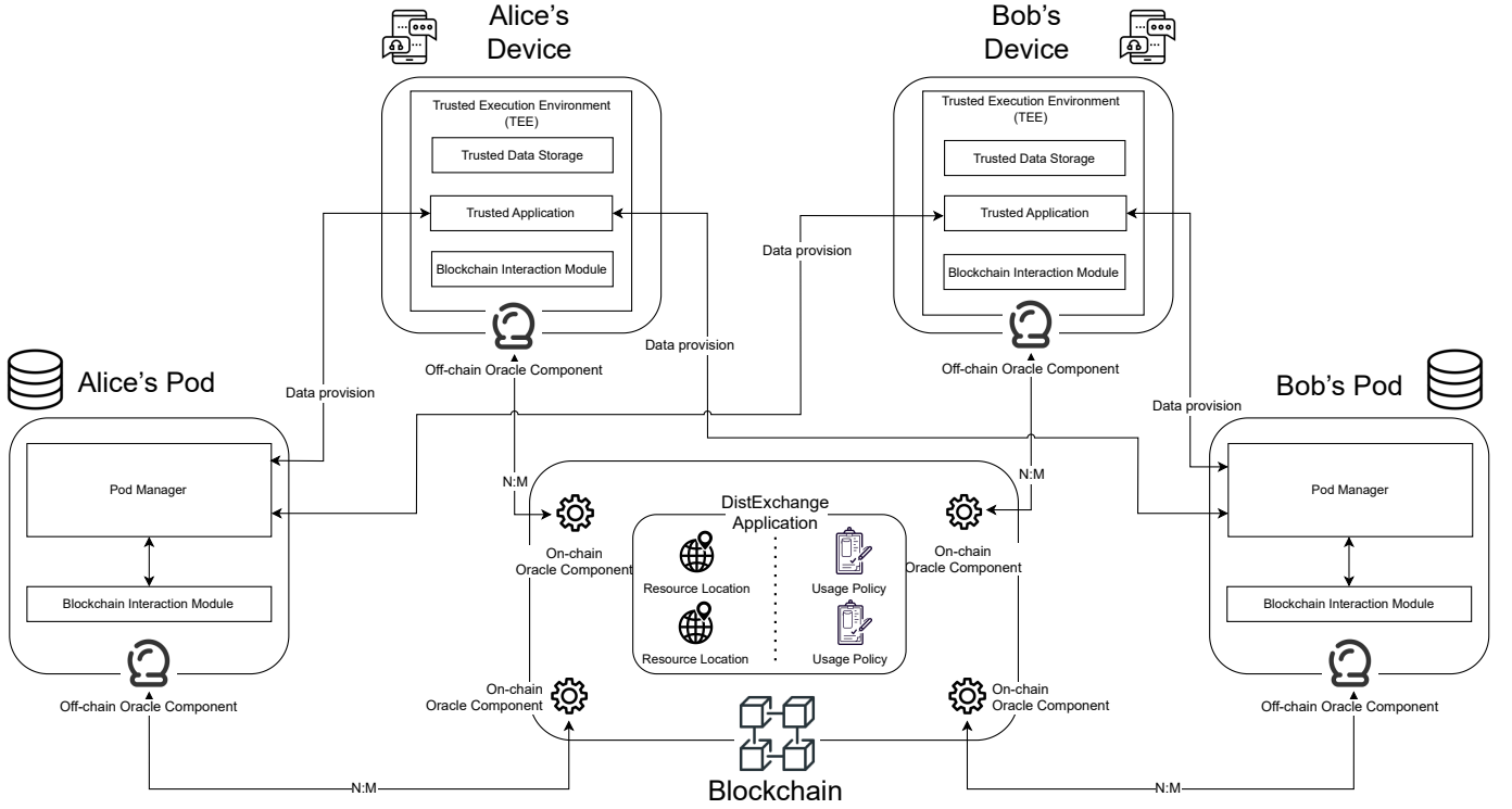
Fig. 1. A Decentralised Usage Control Architecture
