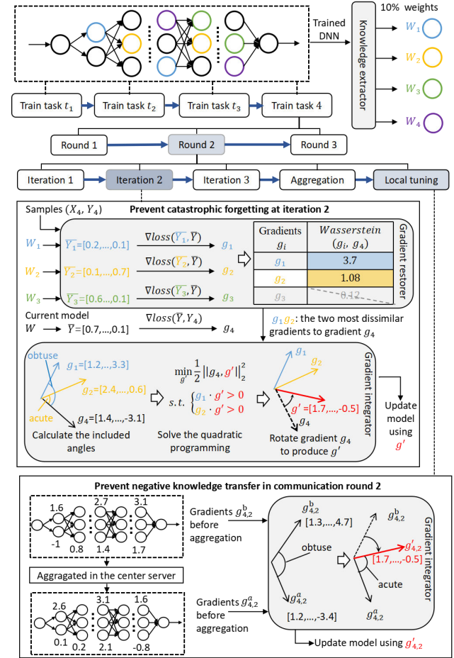
Fig. 3. Example model learning process with FedKNOW
