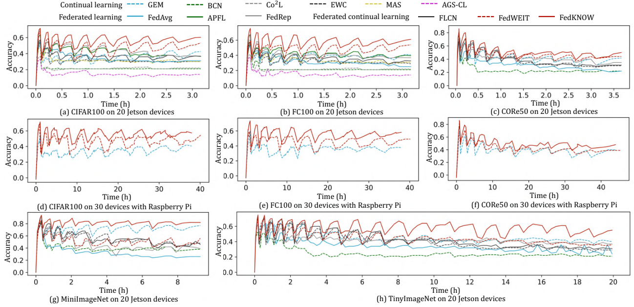
Fig. 4. Comparison of model accuracy and training time between FedKNOW and 11 baseline methods
