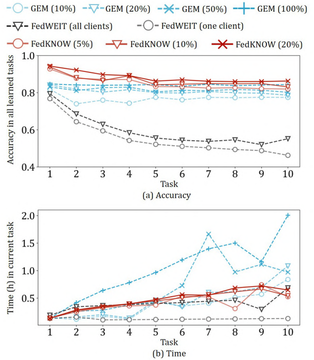
Fig. 10. Discussion of different parameter settings
