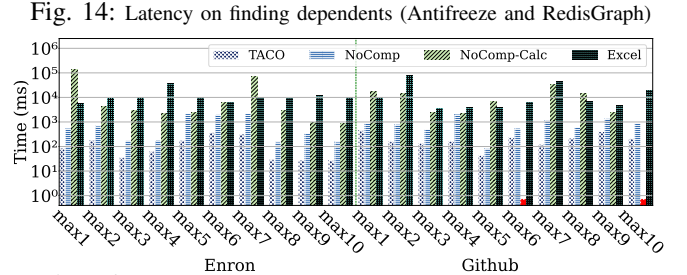
Fig. 14: Latency on finding dependents (Antifreeze and RedisGraph)
