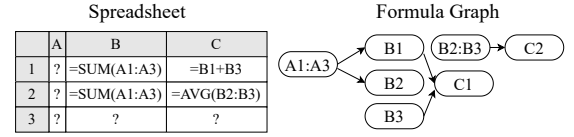
Fig. 3: An example spreadsheet and its formula graph
