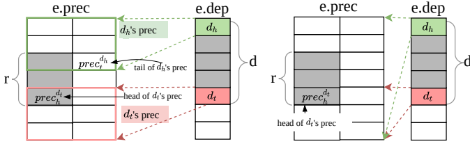
Fig. 6: An example of \text{findDep}(e, r) for RR
