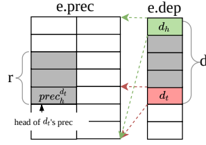
Fig. 7: An example of \text{findDep}(e, r) for RF
