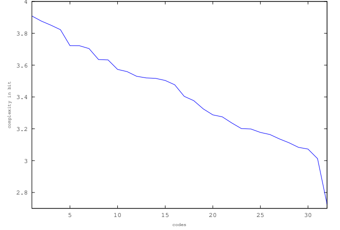
Fig. 4. Complexity values of the 32 codes (sorted) of the codebook illustrated previously (time scale 250 ms learned on 2008 union 2009). The difference between highest and lowest complex codes is significant.
