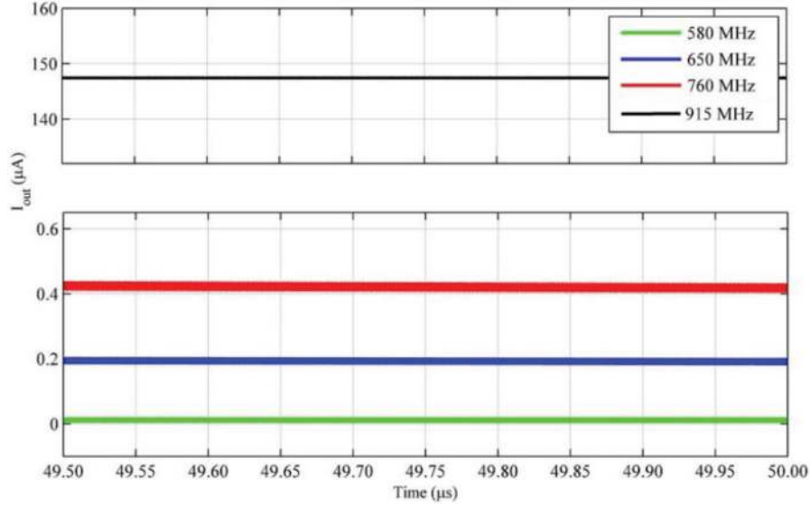
Figure 14. Output currents in 580, 650, 760 and 915 MHz.
