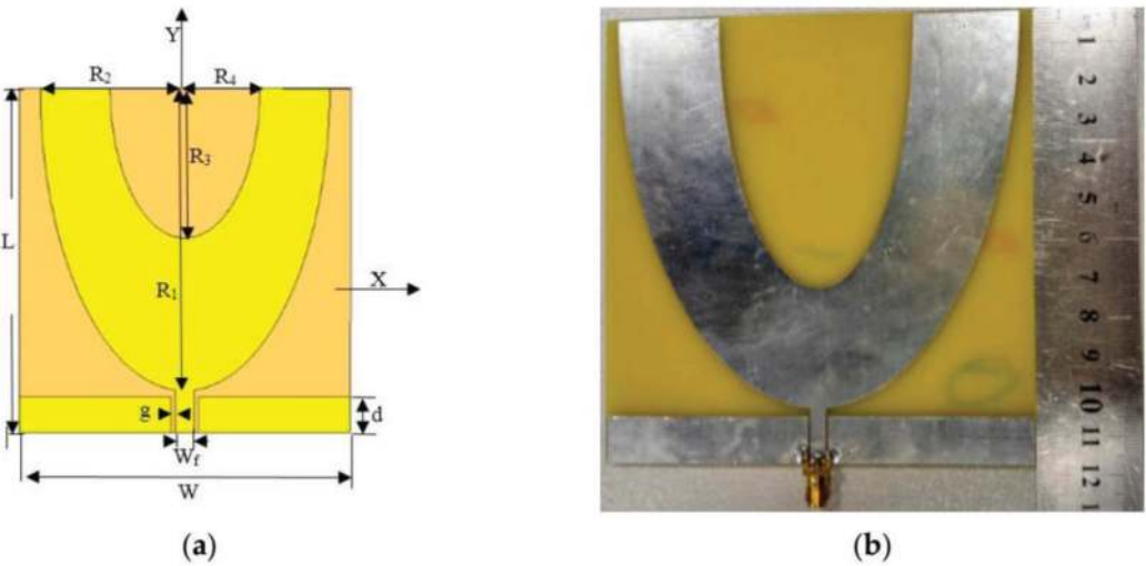
Figure 16. Designed U-shape UWB antenna.
