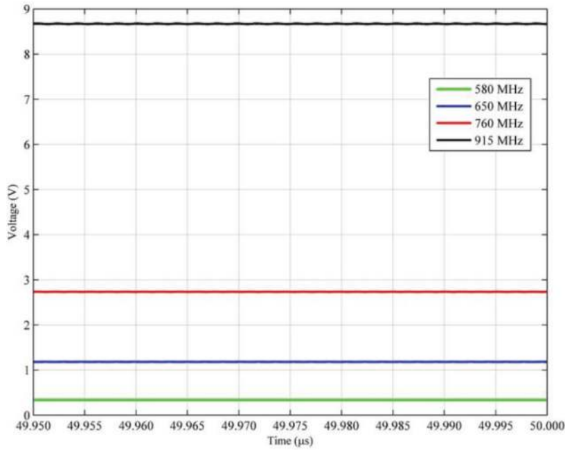
Figure 11. Voltage multiplier circuit output.
