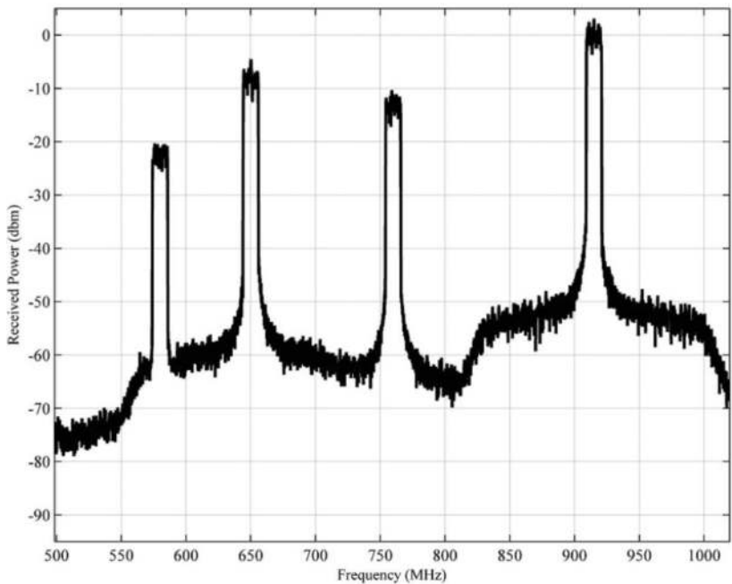
Figure 4. Frequency response of OFDM transmitter in our frequency band with QPSK modulation in receiver end.
