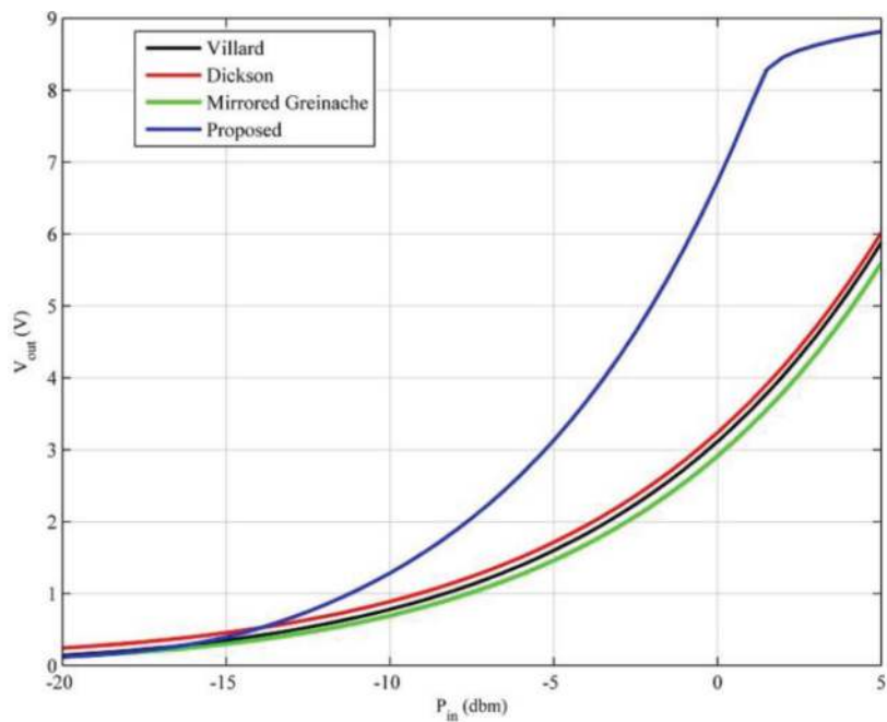
Figure 12. Output voltage versus input power.
