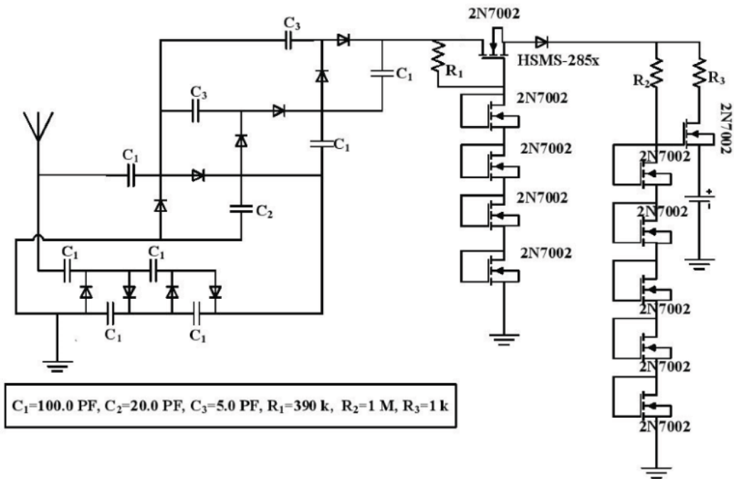
Figure 13. Charger circuit.
