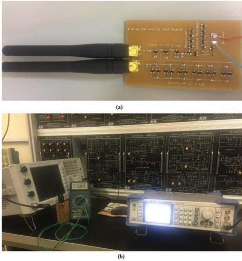
Figure 18. (a) Fabricated charger circuit (b) Circuit test.
