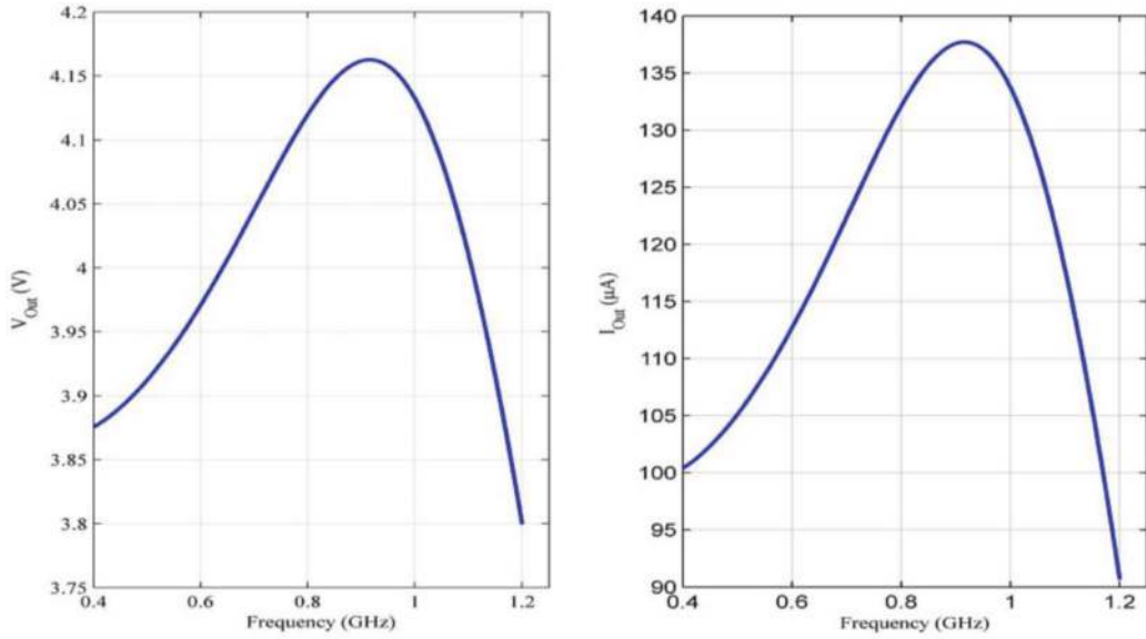
Figure 10. Rectifier circuit output voltage and current.
