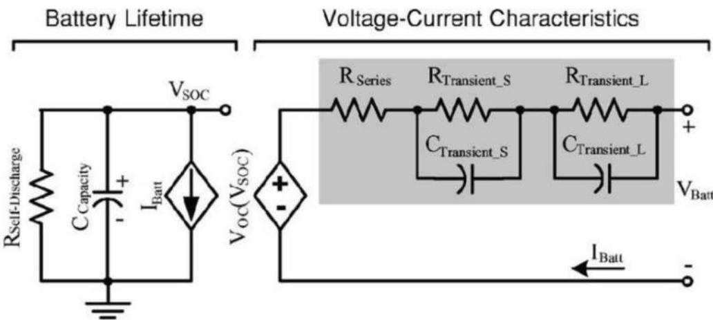
Figure 3. Battery model [34].
