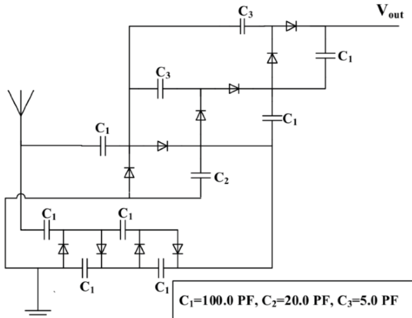
Figure 7. Proposed voltage multiplier circuit.
