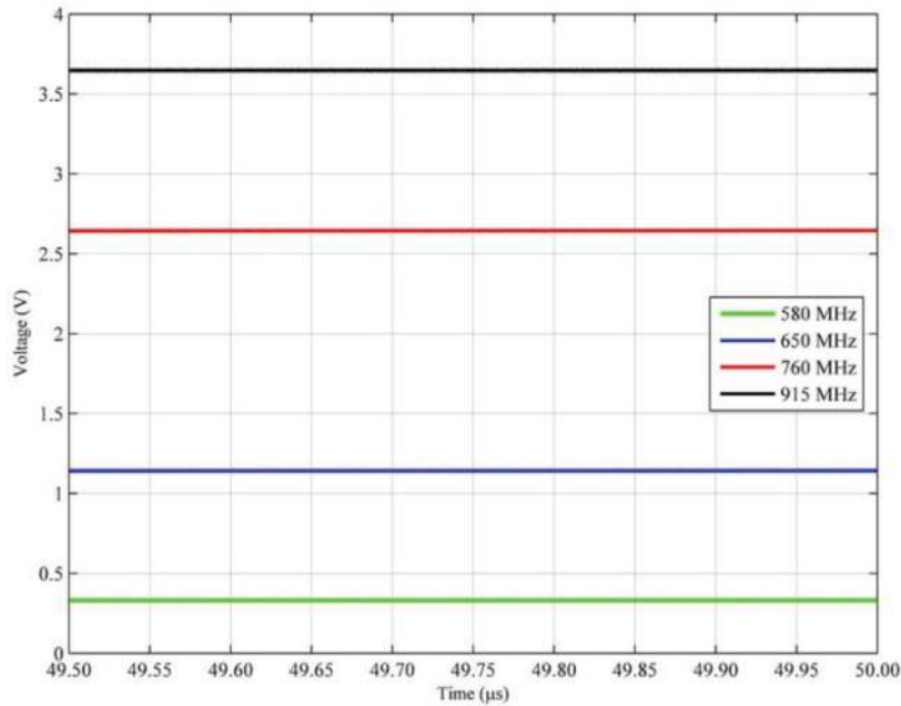
Figure 15. Output voltages in 580, 650, 760 and 915 MHz.
