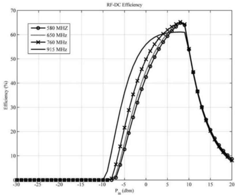
Figure 8. Rectifier circuit efficiency.
