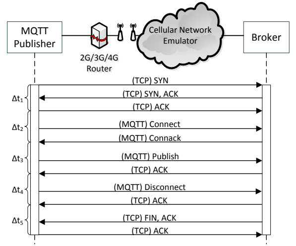
Fig. 6: MQTT data exchange (Payload 2500 bytes)
