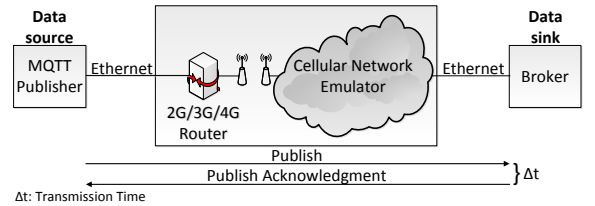
Fig. 4: Test setup for MQTT
