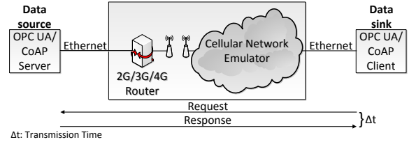
Fig. 3: Test setup for OPC UA and CoAP
