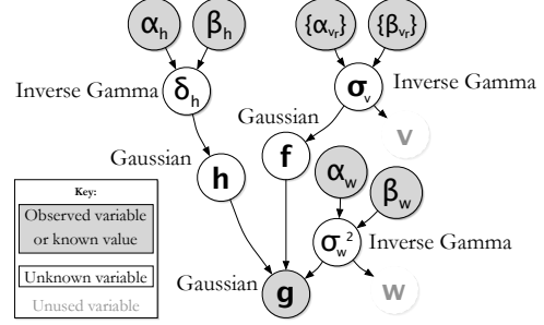
Fig. 2. Graphical model showing relationships between variables
