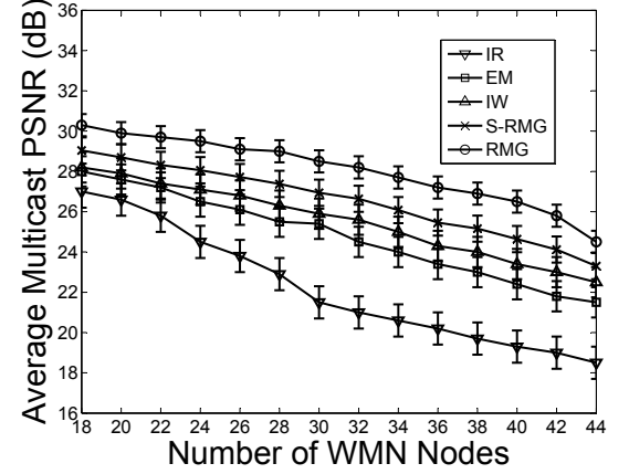
Fig. 10. The average PSNR performance when the WMN size in Fig. 6 increases from 18 to 44.
