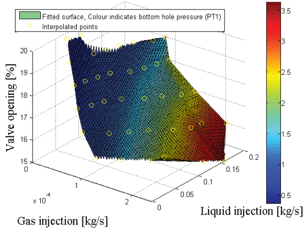
Figure 7. A 3D-plane of the combined flow and bifurcation map. The surface is indicating the plane where stable flow switches to slug flow and the color is indicating the pressure in the bottom of the riser.
