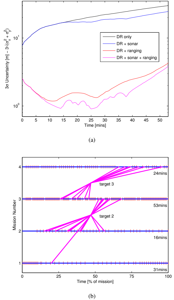
Fig. 6. (a): Navigation uncertainty for Mission 3 for four different algorithm configurations. As expected the dead reckoning-only solution suffers from continuous uncertainty growth (black). When sonar targets are observed, uncertainty growth can be halted using loop closures, before returning to dead reckoning (blue). Acoustic ranging alone can bound error growth — subject to observability (red); while the full sensor fusion produces the solution with minimum uncertainty (magenta). See Sec. 6(a) for more details. (b): During the four (consecutive) missions, range measurements (represented by the red lines) were frequently received from the ASV (Mission 1 and 2) or the research vessel (Mission 3 and 4). Occasionally targets were detected in the side-scan sonar data. Repeated observations of the same target (illustrated in magenta) allow for a SLAM loop closure and for inter-loop uncertainty to be bounded. Note that multiple observations of the same targets occur across the four missions enabling multi-session mapping. Finally, the events presented for Mission 3 synchronize with Fig. (a).
