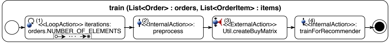
Fig. 1: The behavior of TeaStore's "Recommender.train" service using SEFF
