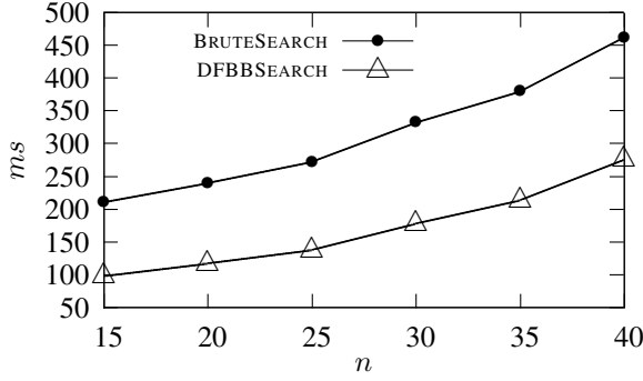
Fig. 3. BRUTESEARCH vs. DFBBSEARCH problems with number of consistent solutions \sim 1000 , average time in ms on y -axis, number of variables n on x -axis.
