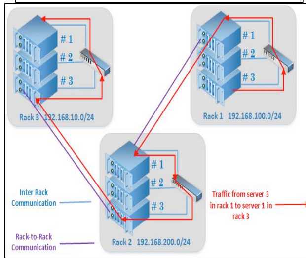
Figure 1. Server Centric PON based data centre network architecture [13]
