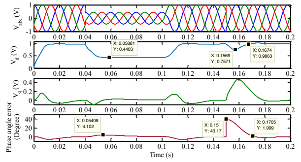
Fig. 4. DDSRF-PLL's performance under the grid fault and 40-degree phase jump.
