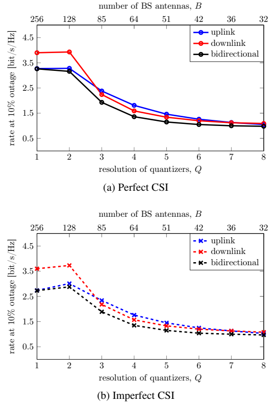
Fig. 5. Uplink, downlink and bi-directional link rates at 10% outage probability with MR precoding and combining. Both perfect CSI and estimated CSI are considered; \rho_{ul} = 5 dB and \rho_{dl} = 15 dB.
