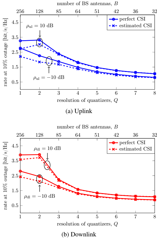
Fig. 4. Uplink and downlink rates at 10% outage probability with MR precoding and combining.
