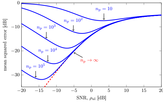
Fig. 3. MSE vs. SNR for the Busgang MMSE channel estimator with different pilot-sequence lengths; 1-bit quantization, B = 100 , U = 1 , and i.i.d. Rayleigh-fading channel.
