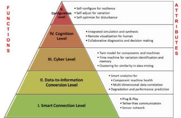
Fig. 2. 5C architecture for implementation of CPSs [2]
