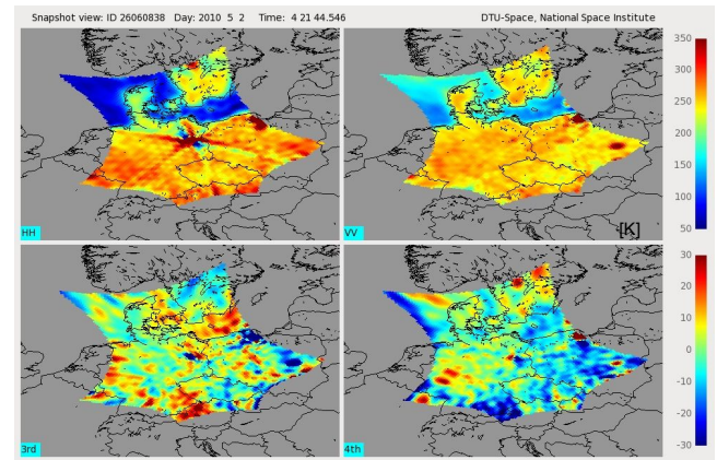
Figure 5: SMOS snapshot, fully polarimetric
