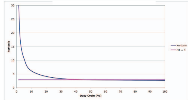
Figure 2: Blind spot, good sensitivity at low duty cycles, and poor sensitivity to large duty cycles
