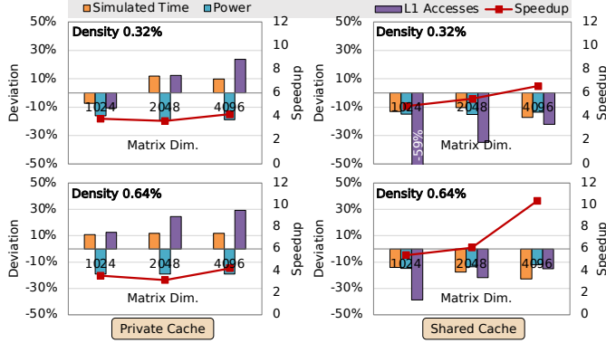
Fig. 9. Accuracy of performance, power and L1 cache access count estimations of HETSIM model compared to the detailed gem5 model of 2 \times 8 Transmuter, for SpMM with varying matrix dimension and density (uniform random), and two HETSIM configurations.
