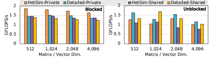
Fig. 11. Strong scaling performance comparison between different 2 \times 8 Transmuter configurations on two GeMV implementations, using HETSIM and the detailed model.
