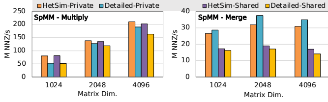
Fig. 12. Strong scaling performance comparison between different 2x8 Transmuter configurations on an SpMM outer product implementation with uniform random matrices, using HETSIM and the detailed model.
