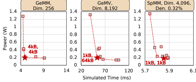
Fig. 13. Pareto analysis for GeMM, GeMV and SpMM on 4x16 Transmuter. The datapoints correspond to \text{Cap}_{L1} \in \{1, 4, 16, 64\} kB, \text{Cap}_{L2} \in \{1, 4, 16, 64\} kB, \text{Cap}_{L1} \leq \text{Cap}_{L2} . Star indicates the design with best energy-efficiency.
