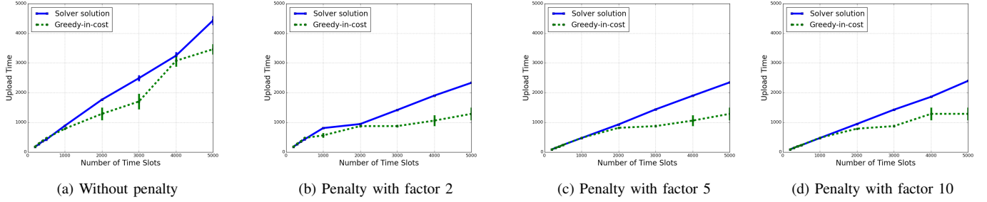
Fig. 6: Upload Time
