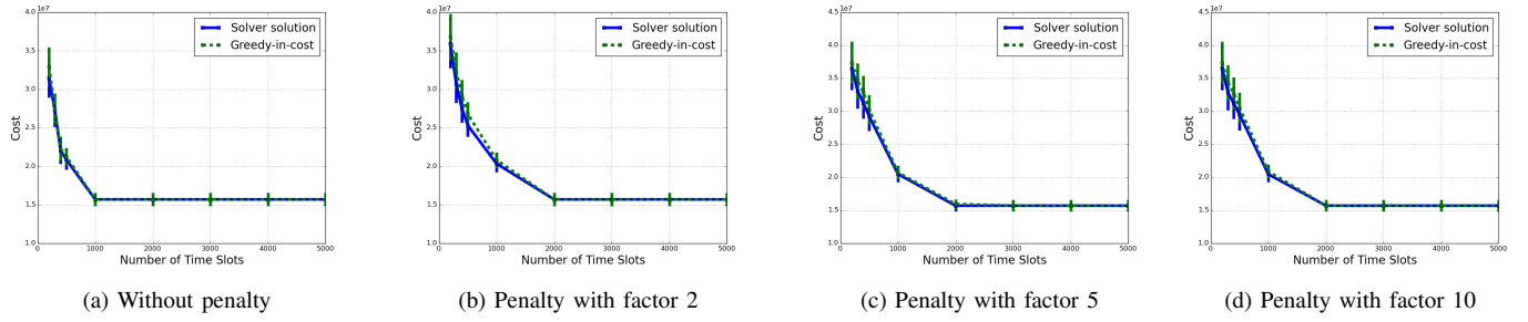
Fig. 5: Cost
