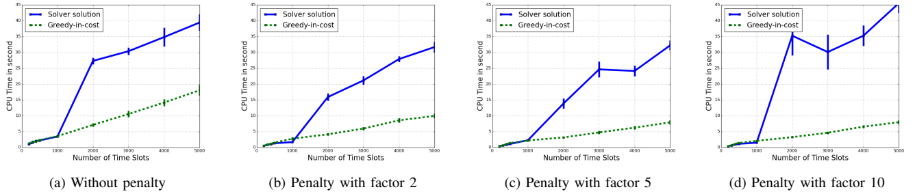
Fig. 7: CPU Time
