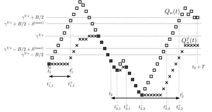
Fig. 6. Partitioning \mathcal{T}_L(T) into intervals of t_k , t_k' , t_{k,j}^- , and t_{k,j}^+ .
