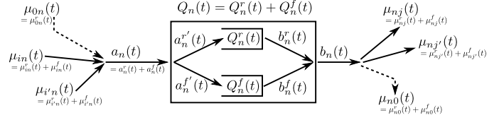
Fig. 3. Transformation of a standard queue to a floating queue
