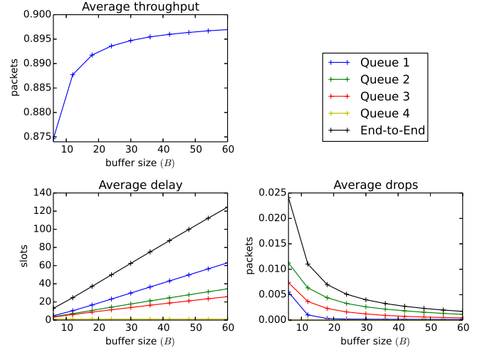
Fig. 9. Results of throughput maximization problem with V = 200
