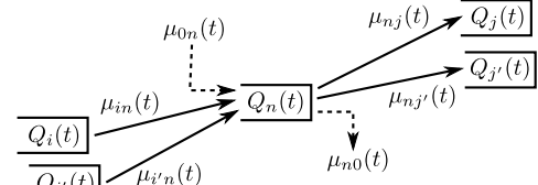
Fig. 1. Arrivals and services at a standard queue
