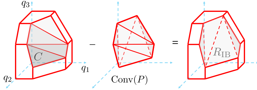
Fig. 3. Visualizing R_{IB} for the three-user scenario in Figure 2. In this example, the expected payoff vectors P = \{\mathbf{p}(\mathbf{d}) | \mathbf{d} \in D\} are not on the same hyperplane and R_{IB} = \text{cl}(C - \text{Conv}(P)) .
