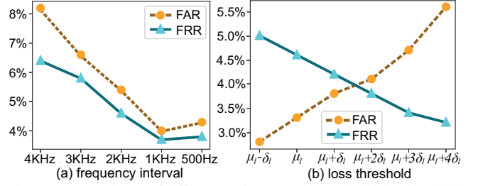
Fig. 14. FRR and FAR of different (a) frequency intervals, (b) loss thresholds
