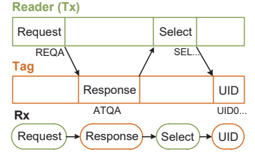
Fig. 2. The communication process between NFC reader and tag of the ISO/IEC 14443 Type A and B standard.
