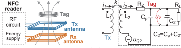
Fig. 3. Setting to capture request and response signal
