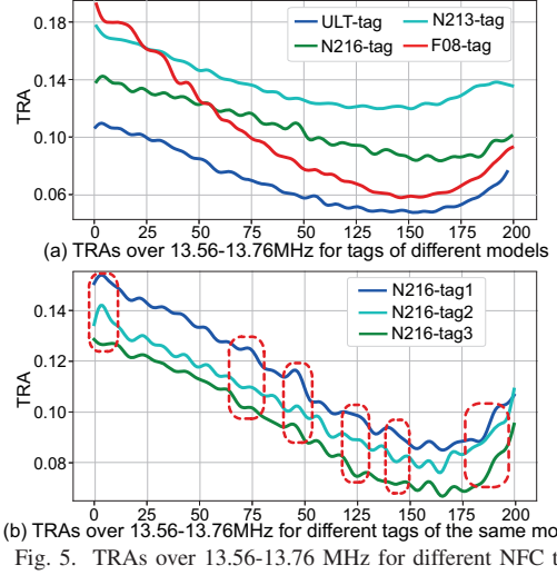
Fig. 5. TRAs over 13.56-13.76 MHz for different NFC tags
