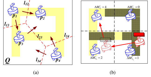
Fig. 1. Example of the equal-mass partitioning and delivery by the gradient of the demanding mass. 4 mobile manipulators (assembly robots) are displayed in a convex region Q that includes the A-shaped target structure. The yellow region has high density \phi_t . The mass of a robot is the size of the total yellow region in its partition (Voronoi region.) p_i ( i = 1, 2, 3 ) denotes the position of the assembly robots and the red-dotted lines l_{ij} are shared boundaries of the partitions between two robots. \Delta M_{V_i}^t is the demanding mass.
