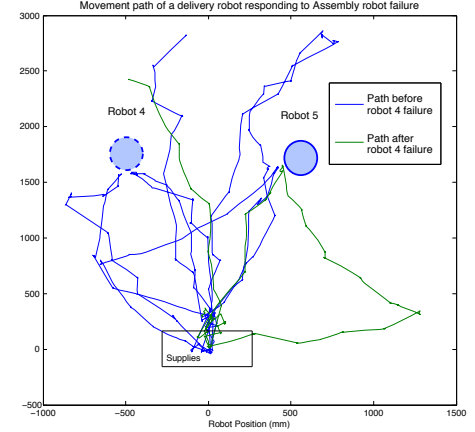
Fig. 12. Adaptive behavior of the system: a delivery robot begins by delivering parts fairly to robot 4 and robot 5. When robot 4 (on the left) fails in the middle of the test, the delivery robot begins delivering only to robot 5.
